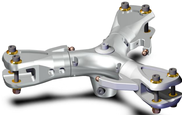
HELIOS 3-Blatt-Rotorkopf / 3-Bladed Main Rotor
